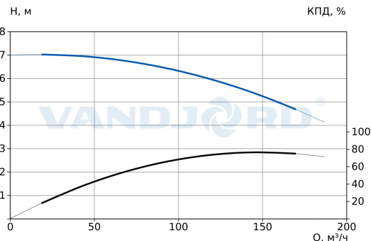
73319023 VNK 200-150/230 Q-A-E-B-AB-E
