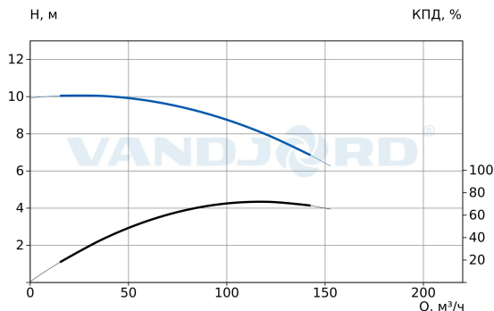
73318030 VNK 150-125/259 Q-A-E-B-AB-E
