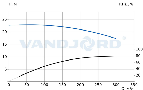
73319013 VNK 200-150/262 Q-A-E-B-AB-E
