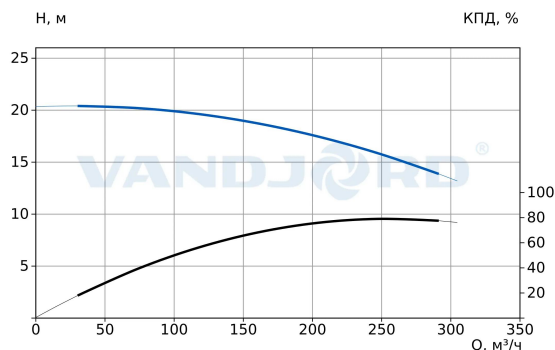
73319011 VNK 200-150/257 Q-A-E-B-AB-E
