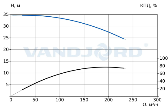
73318025 VNK 150-125/316 Q-A-E-B-AB-E
