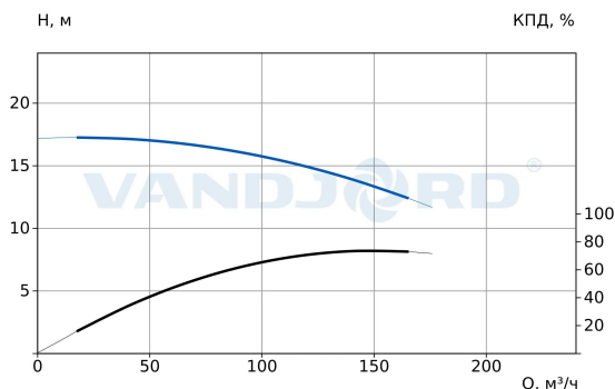
73318021 VNK 150-125/225 Q-A-E-B-AB-E
