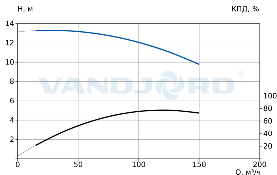
73318019 VNK 150-125/215 Q-A-E-B-AB-E
