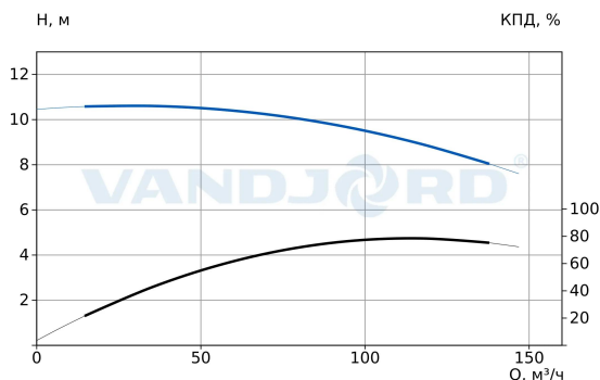
73318018 VNK 150-125/192 Q-A-E-B-AB-E
