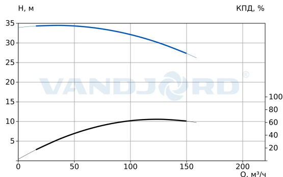
73317029 VNK 125-100/318 Q-A-E-B-AB-E
