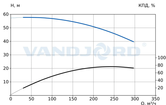
73318006 VNK 150-125/219 Q-A-E-B-AB-E
