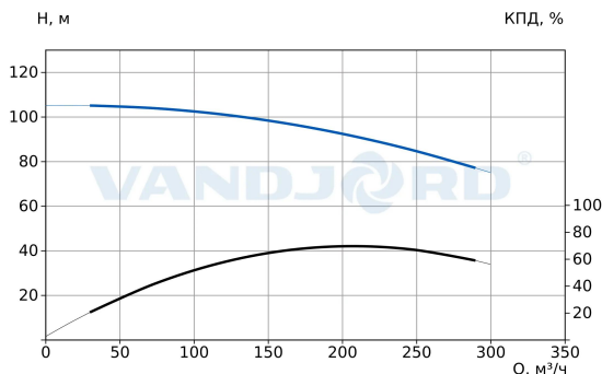
73317015 VNK 125-100/283 Q-B-E-B-AB-E
