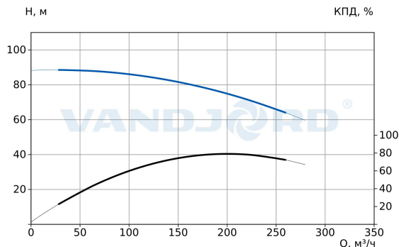
73317013 VNK 125-100/254 Q-A-E-B-AB-E
