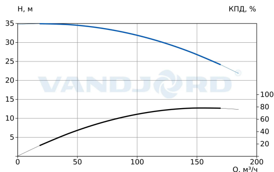
73317005 VNK 125-100/166 Q-A-E-B-AB-E
