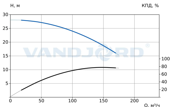
73317004 VNK 125-100/153 Q-A-E-B-AB-E
