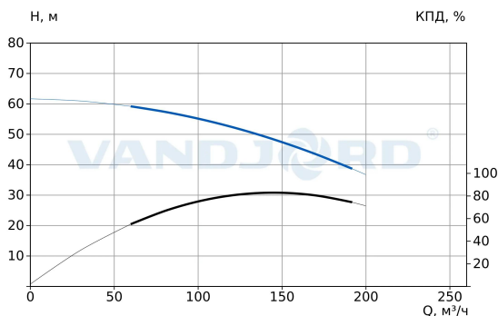
73215089 NBV iNOX 80-200-30/2 CN-A1-D-E-B-A-E
