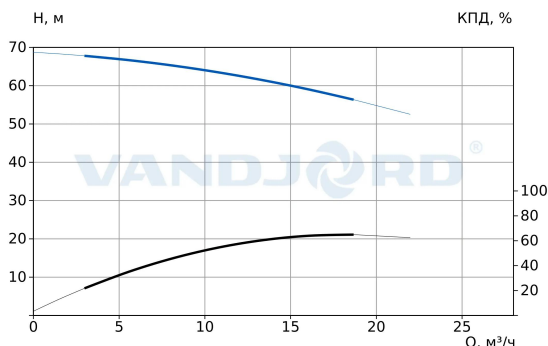
73211039 NBV iNOX 32-200-7.5/2 CN-A1-D-E-B-A-E
