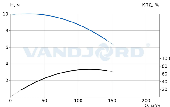
73118156 TPV 125-80-4/6 Q-A-BT-E
