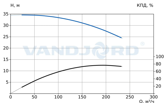
73118151 TPV 125-280-22/4 Q-A-BT-E
