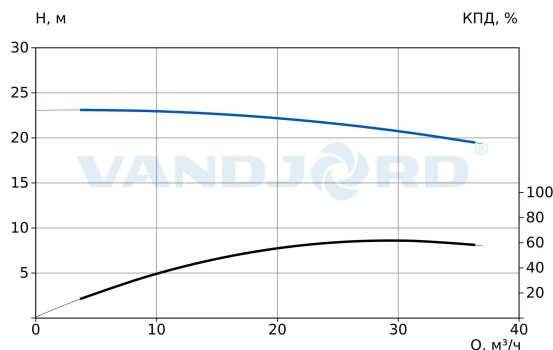
73114134 TPV 50-210-3/4 Q-A-BT-E
