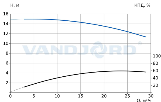
73114132 TPV 50-120-1.5/4 Q-A-BT-E
