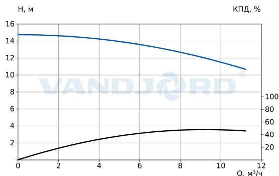
73112109 TPV 32-120-0.75/4 Q-A-BT-E
