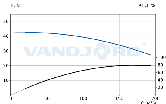
73117138 TPV 100-320-22/2 Q-A-BT-E
