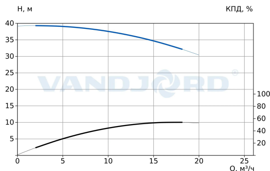
73112114 TPV 32-350-3/2 Q-A-BT-E
