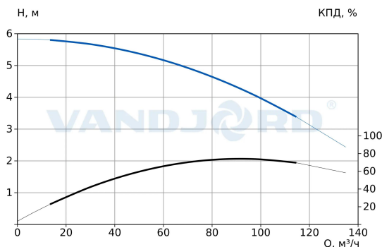
73118124 TPV 125-50-1.5/6 Q-A-B-E
