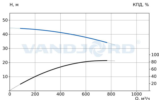
73122113 TPV 250-370-90/4 Q-A-B-E
