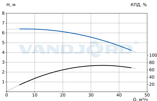
73116117 TPV 80-50-0.75/4 Q-A-B-E
