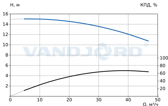
73115115 TPV 65-120-2.2/4 Q-A-B-E
