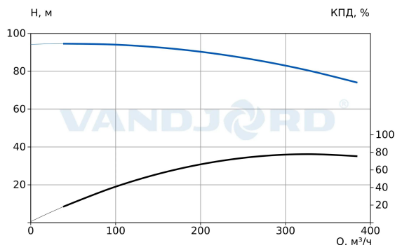
73118108 TPV 125-770-110/2 Q-A-B-E
