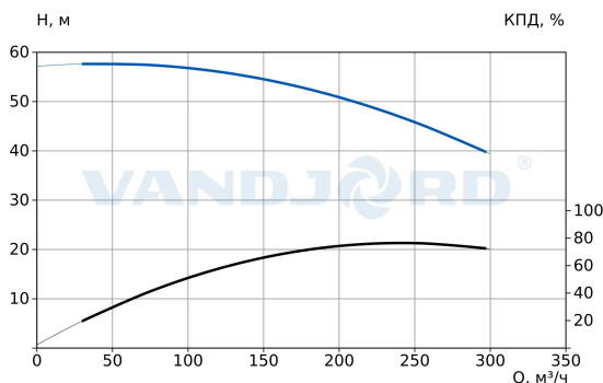
73118104 TPV 125-460-45/2 Q-A-B-E
