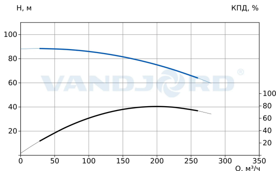
73117113 TPV 100-720-75/2 Q-A-B-E
