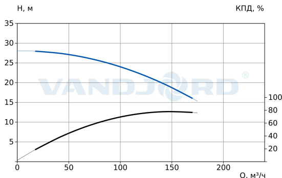
73117104 TPV 100-210-11/2 Q-A-B-E
