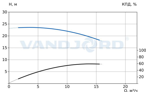
73112104 TPV 32-220-1.5/2 Q-A-B-E
