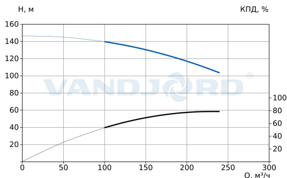
74147015 CRV 200-4-2CN AI-D-E-HUBE-E
