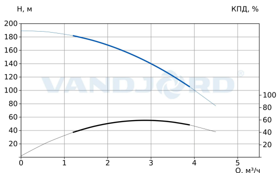
74113764 CRV 3-31C A-D-E-HQQE-E
